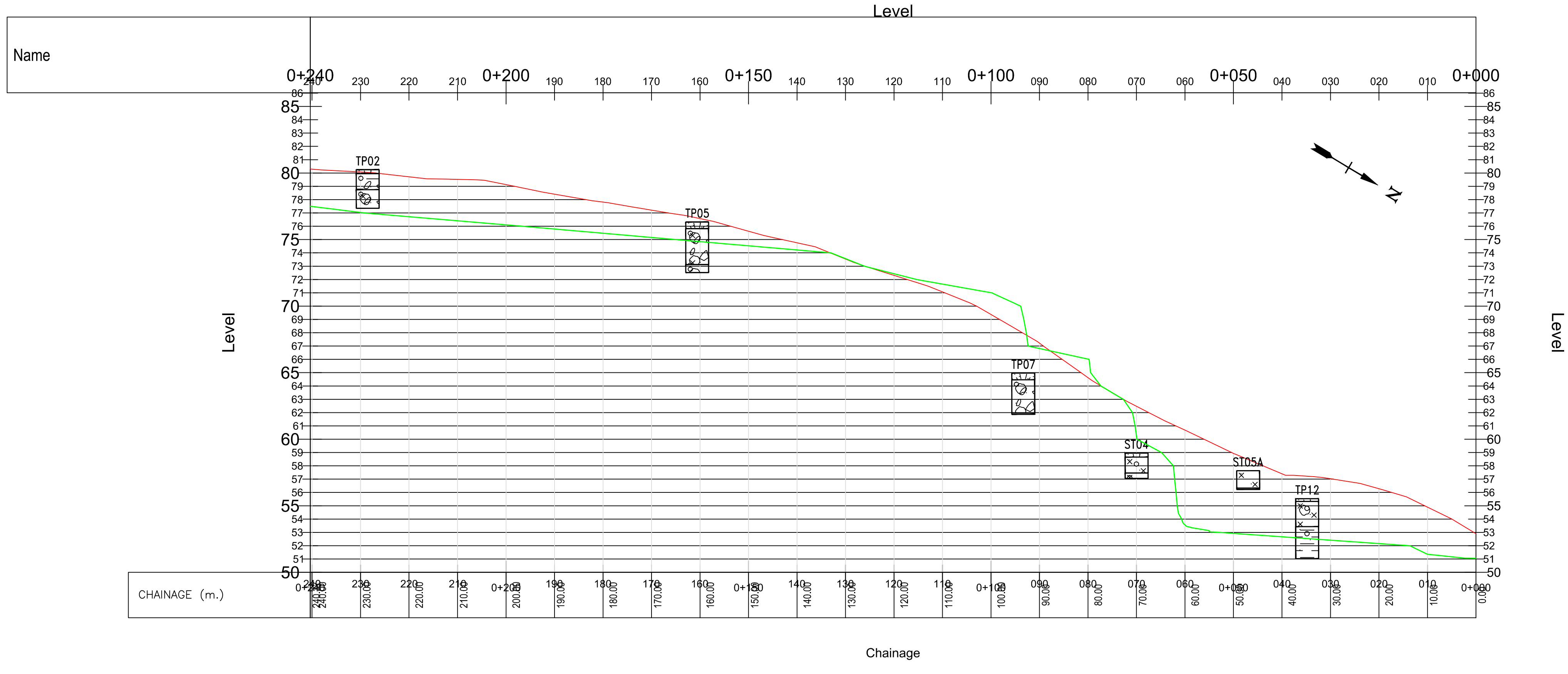
LONGSECTION OF BASELINE 2 - LONGSECTION 2 SCALE: H 1:500, V 1:182. DATUM: 50.000
